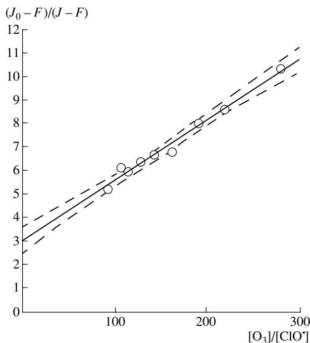
Fig. 2. (J_0 - F)/(J - F) vs. [O_3]/[ClO^\bullet] plot obtained in experiments performed at a constant ozone concentration equal to 4.38 \times 10^{14} molecule/cm 3 and a variable [ClO^\bullet] concentration. The dotted line corresponds to a 98% confidence interval.
